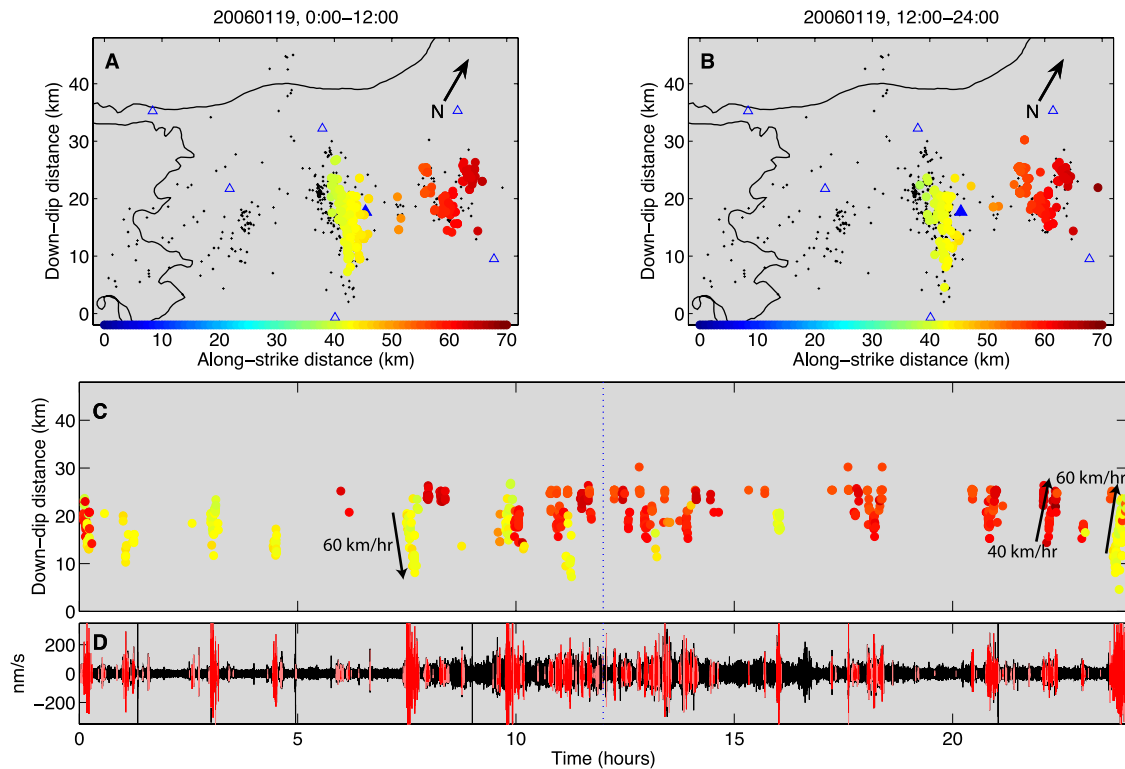
Figure 7. Same as Figure 3, but for 19 January 2006.
