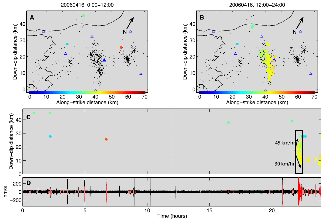
Figure 11. Same as Figure 10, but for 16 April 2006.
