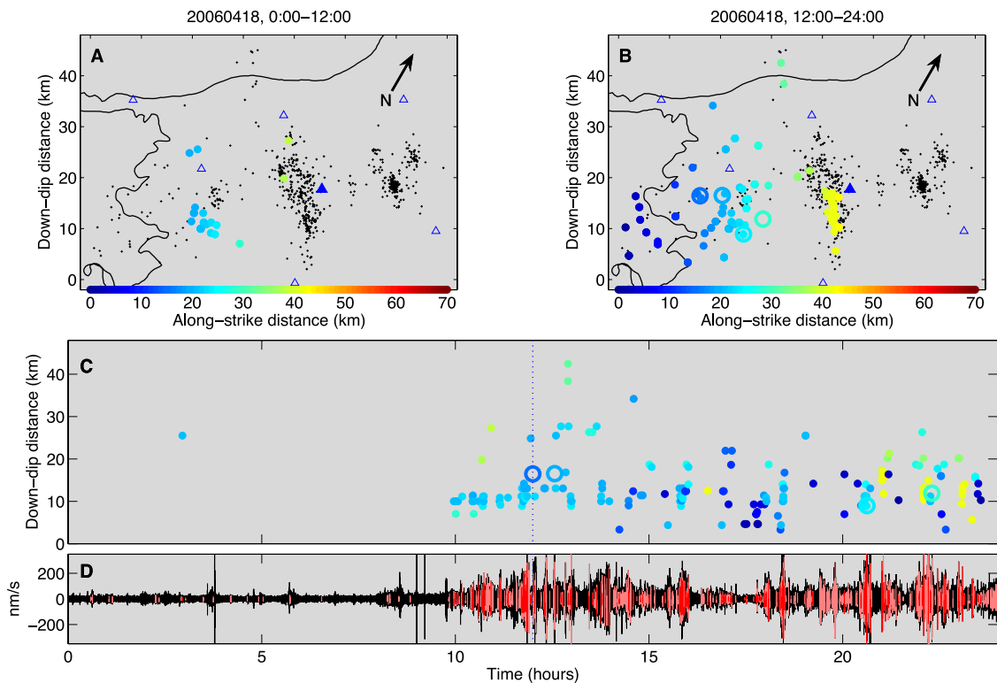
Figure 13. Same as Figure 10, but for 18 April 2006. Large open circles in Figures 13b and 13c indicate the occurrence of VLF events, as reported by Ito et al. [2007].
