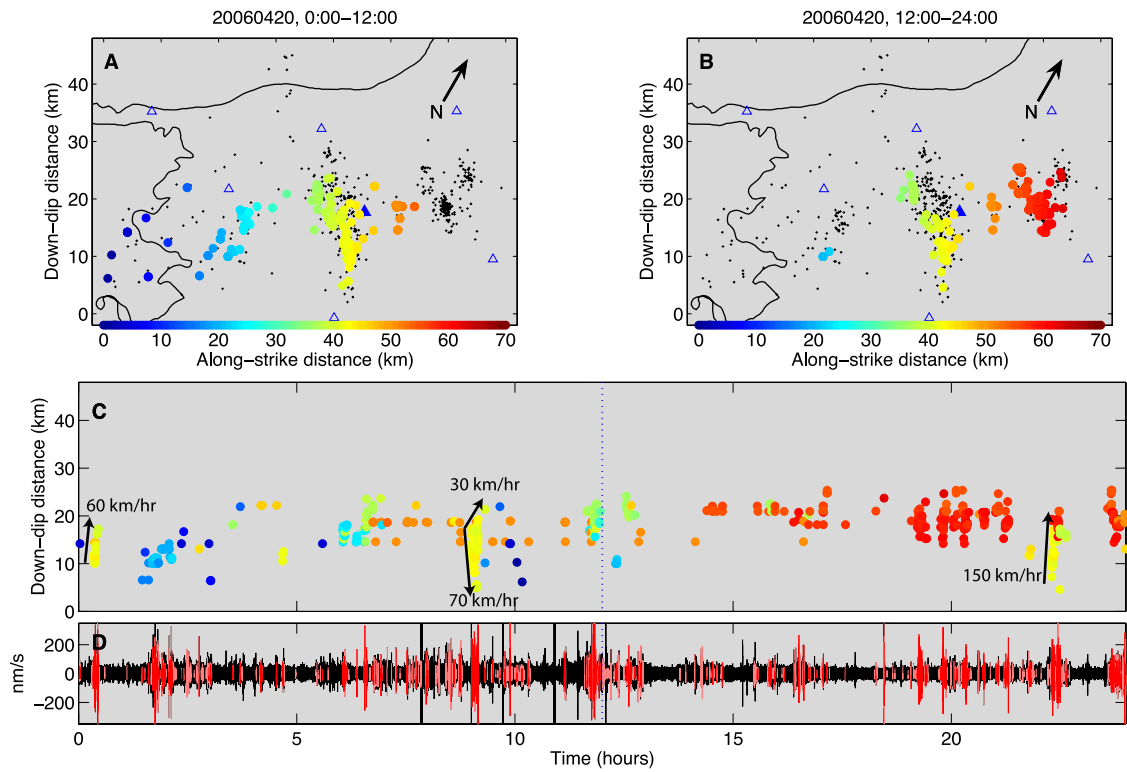
Figure 15. Same as Figure 10, but for 20 April 2006.
