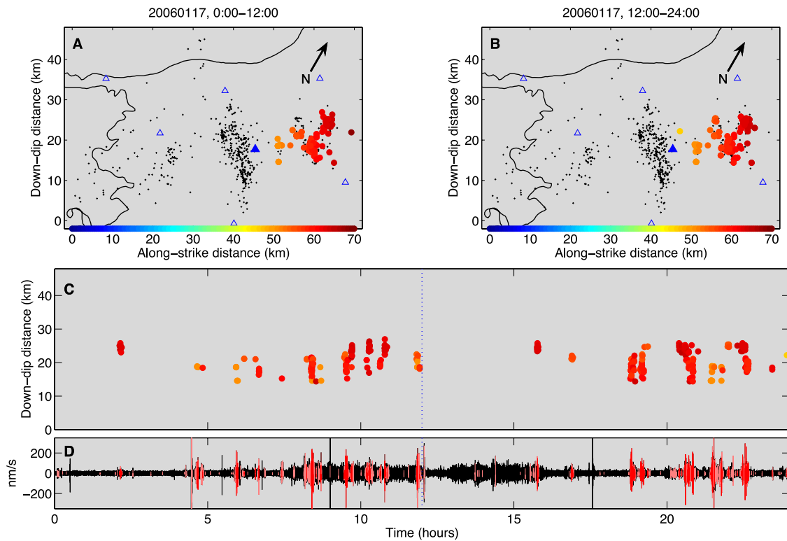
Figure 5. Same as Figure 3, but for 17 January 2006.
