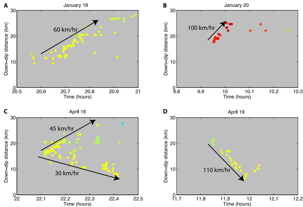
Figure 17. Zoomed view of four migration episodes, plotted as down-dip distance versus time. Each panel shows a 30-min period: (a) 18 January (Figure 6), (b) 20 January (Figure 8), (c) 16 April (Figure 11), and (d) 19 April (Figure 14). These panels demonstrate the variety of migration modes, including updip (Figure 17d), downdip (Figures 17a and 17b), and bilateral (Figure 17c).
