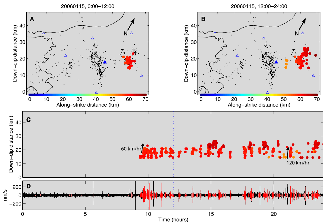
Figure 3. Figures 3–9 show the space-time progression of tremor during 15–21 January 2006. Date is given by figure heading. (a) Map view showing active LFE template events (colored circles) during the first half of each day (0000–1200 LT). The color scale indicates the along-strike position, for reference when comparing with Figure 3c. Only very robust detections exceeding 9^*MAD (see text) are plotted. If multiple detections are present, the strongest in each 2-s window is plotted. Black dots show epicentral locations for LFE template sources. Blue triangles indicate the locations of Hi-net stations used in this study, with the solid triangle showing station N.KWBH referred to in Figure 3d. The black line is the coastline of Shikoku. (b) Same as Figure 3a, but for the second half of each day (1200–2400 LT). (c) Down-dip position of tremor versus time. Events are color-coded by along-strike position as in Figures 3a and 3b. Arrows and labels indicate the direction and approximate migration velocity for some of the clearest examples of migration, as determined by visual inspection of a zoomed view. Notice the migration of tremor that can be seen in both the updip or downdip directions. Black boxes indicate the times and locations of zoomed views in Figure 17. (d) Seismic waveform from station N.KWBH, north component (location shown in Figure 3a). Portions of the waveform plotted in red indicate times of very robust detections (exceeding 9^*MAD ), while portions plotted in pink indicate times with standard detections (exceeding 8^*MAD ; see text for details). A relatively steady, low-amplitude signal seen around midday and uncorrelated with LFEs does not appear to be nonvolcanic tremor, as neighboring stations do not record a similar signal.
