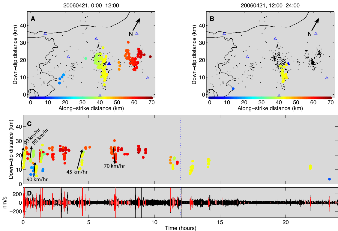
Figure 16. Same as Figure 10, but for 21 April 2006.
