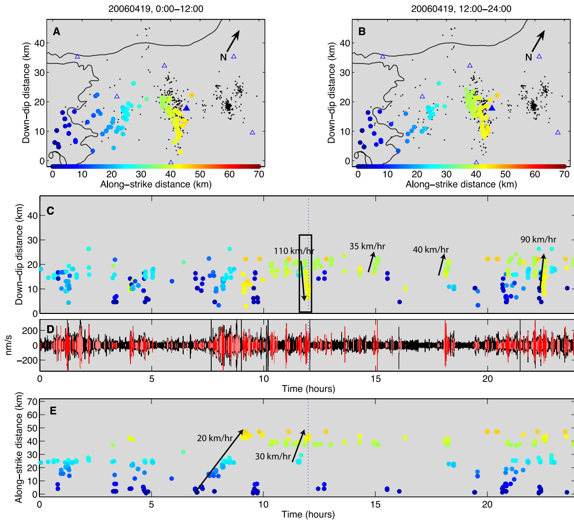
Figure 14. Same as Figure 10, but for 19 April 2006. Figure 14e shows the along-strike position of tremor versus time.
