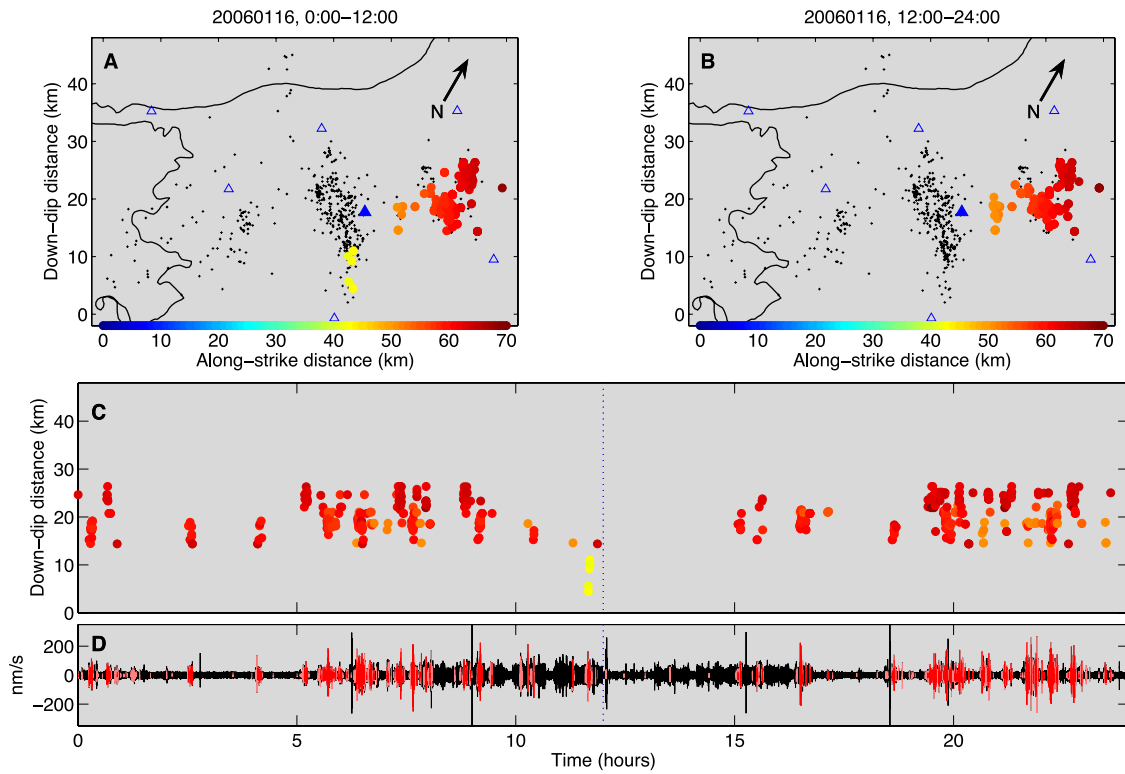
Figure 4. Same as Figure 3, but for 16 January 2006.
