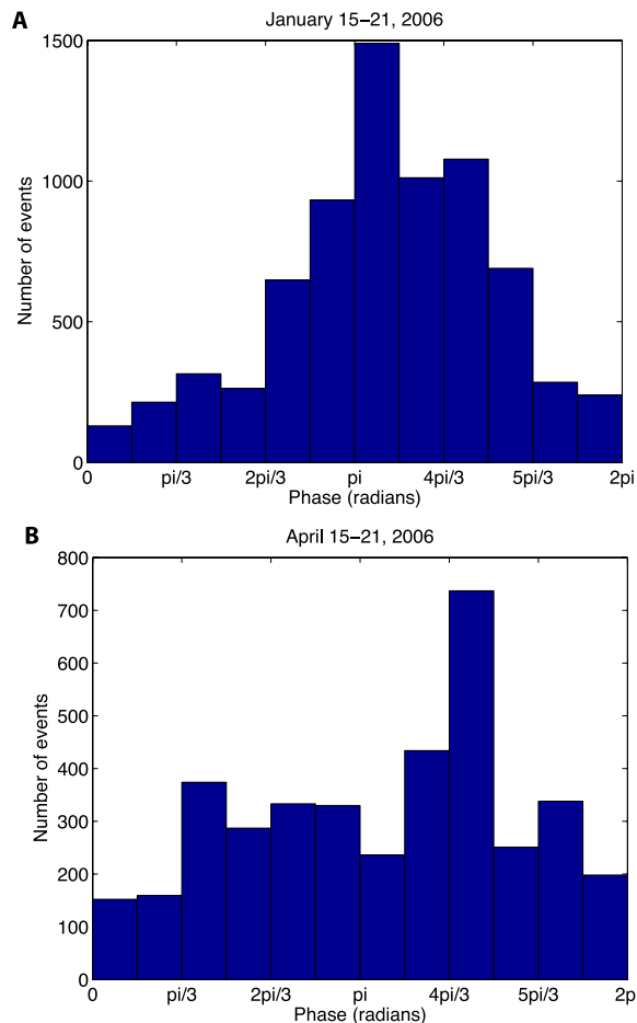
Figure 19. Histograms of LFE numbers versus phase angle, assuming a period of 12.4 hours (the average tidal period): (a) 15–21 January 2006 and (b) 15–21 April 2006. The phase angle is assigned to be zero at the beginning of each episode (i.e., at 0000 LT on 15 January and 15 April) and is repeated every 12.4 hours. The January event exhibits a very clear tidal triggering, while the tidal effect in the April event is less obvious.
