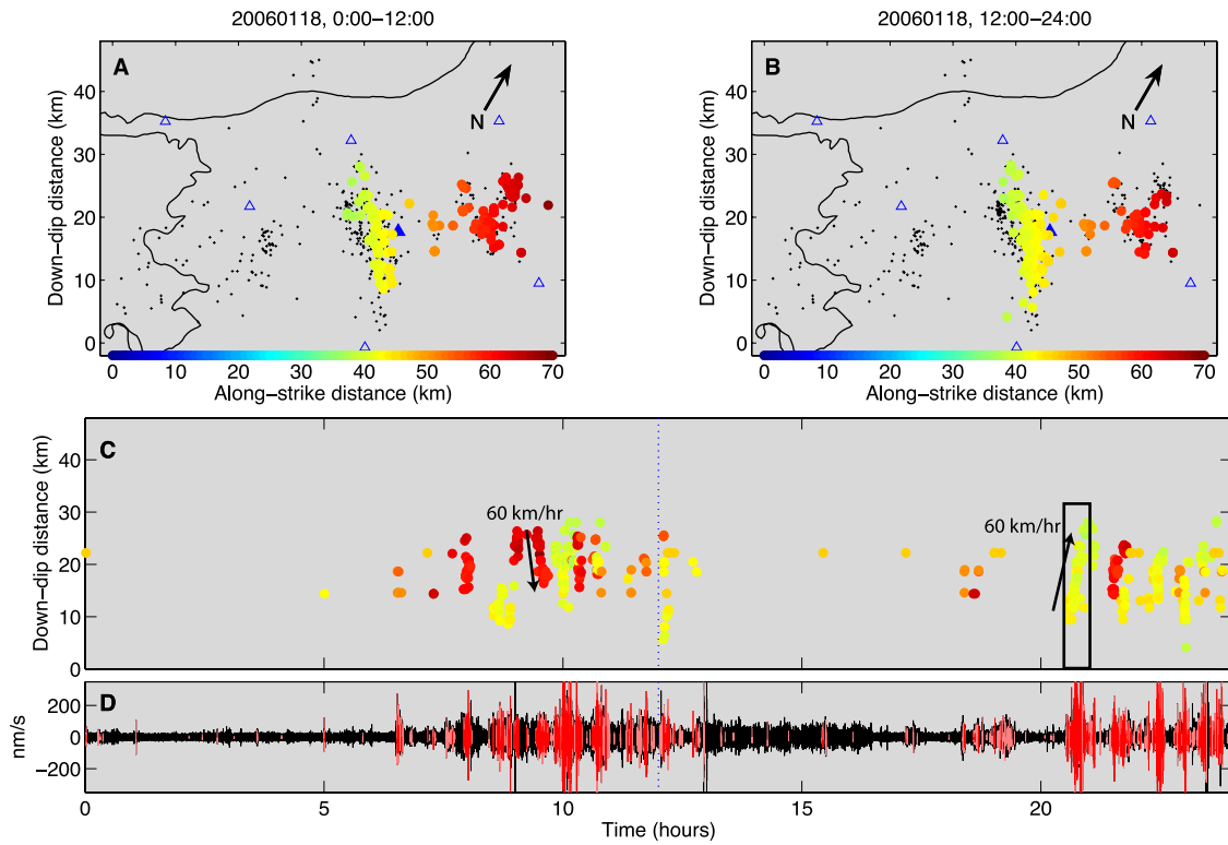
Figure 6. Same as Figure 3, but for 18 January 2006.
