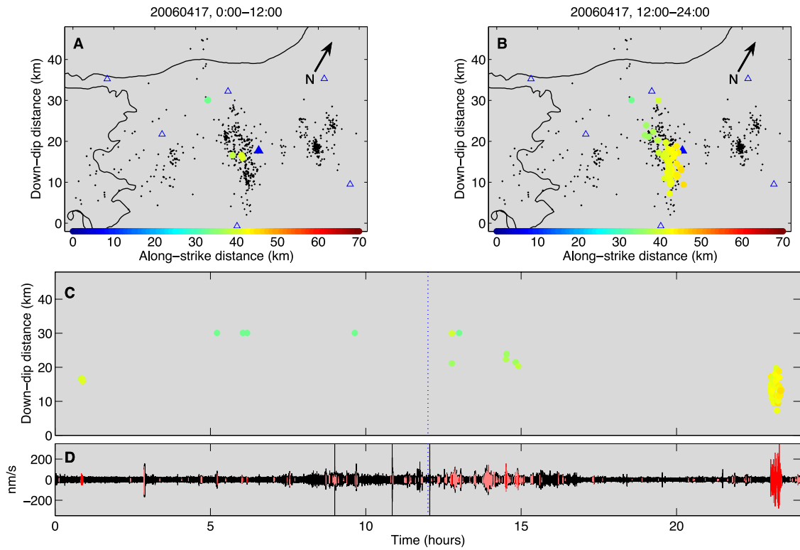
Figure 12. Same as Figure 10, but for 17 April 2006.
