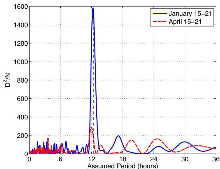
Figure 18. Evidence for tidal triggering of LFE activity. The population of detected LFEs during each tremor and slip episode is analyzed for nonrandomness at periods from 0.2 to 36 hours. The quantity D^2/N relates to the statistical significance of the nonrandomness in Schuster's test (see text). The January event (solid blue line) exhibits an extremely strong periodicity near the average tidal period of 12.4 hours (dashed black line). Tidal triggering in the April event (dashed red line) is less obvious, but this episode still shows a periodicity very close to the average tidal period.
