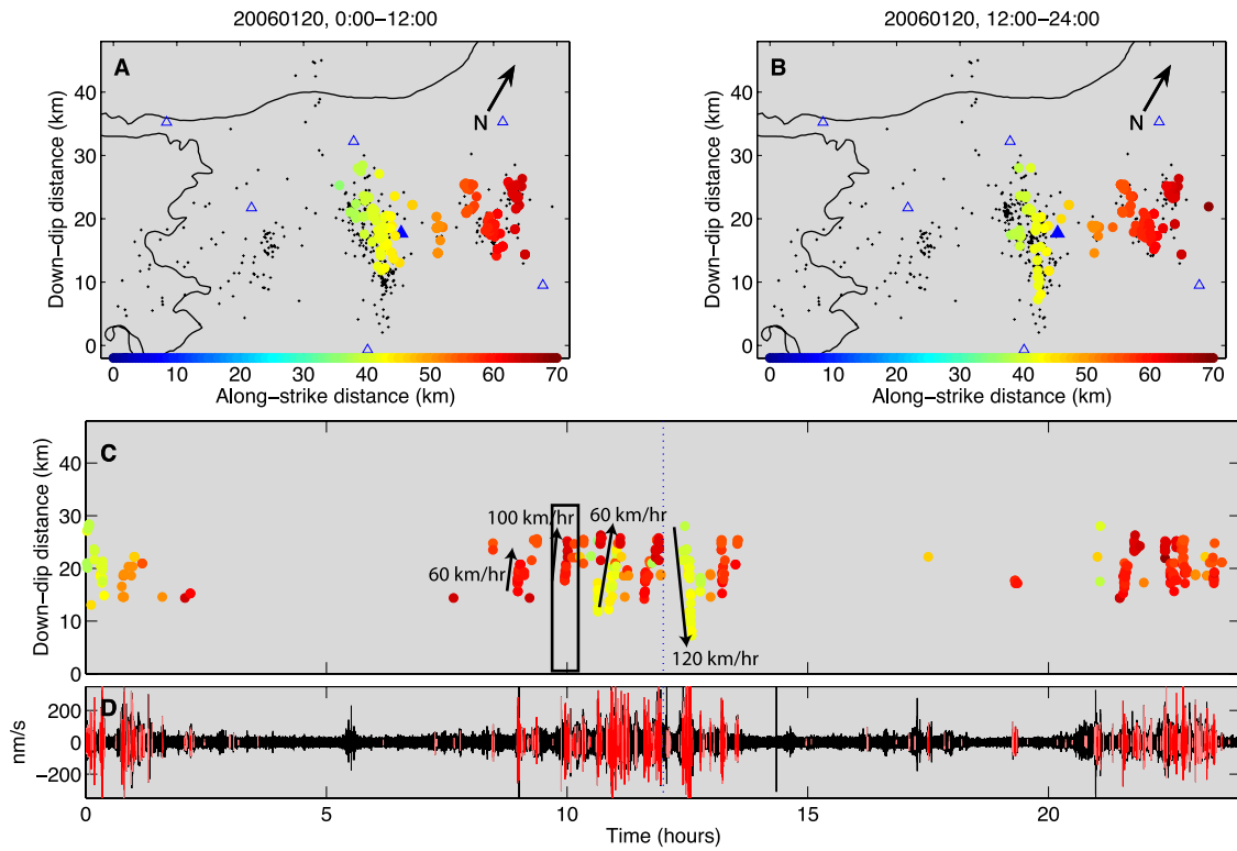
Figure 8. Same as Figure 3, but for 20 January 2006.
