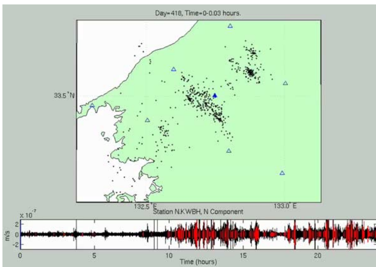
Animation 2. Same as Animation 1, but for the period from 15–21 April 2006. Animation available in the HTML.
