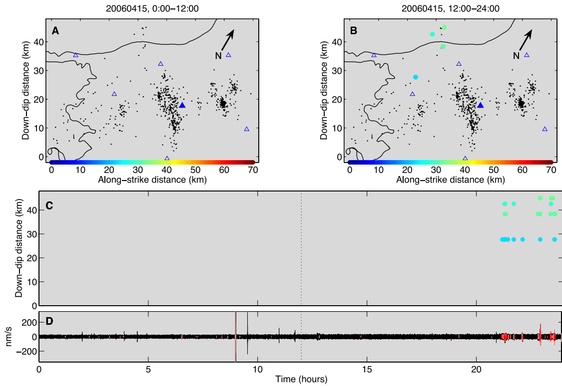
Figure 10. Figures 10–16 are the same as Figures 3–9, but for 15–21 April 2006.
