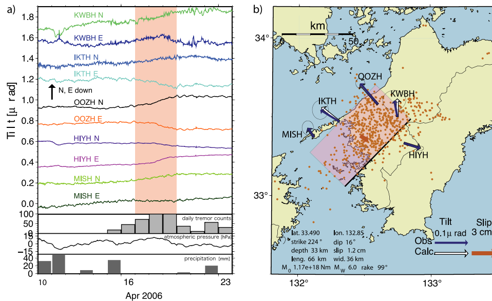
Figure 2. The April 2006 tremor and slip event. (a) From top to bottom: time series of tiltmeter records, daily tremor counts, atmospheric pressure, and precipitation from 10–24 April 2006. Station names and components are given next to each tiltmeter record. The records are plotted after removing their linear trend and estimated tidal and atmospheric components (figure from Sekine and Obara [2006]). (b) Tilt change vectors (blue arrows; ground downward direction), the estimated short-term slow slip model (red rectangle area and arrow) from these tilt change data, and the calculated tilt changes due to this short-term slow slip event model (open arrows) for the western Shikoku region. Epicenters of deep low-frequency tremor activity are also plotted during the same time period (17–20 April 2006) (figure from Sekine and Obara [2006]).
