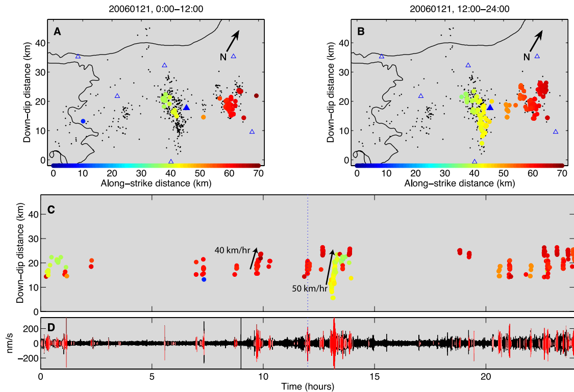
Figure 9. Same as Figure 3, but for 21 January 2006.
