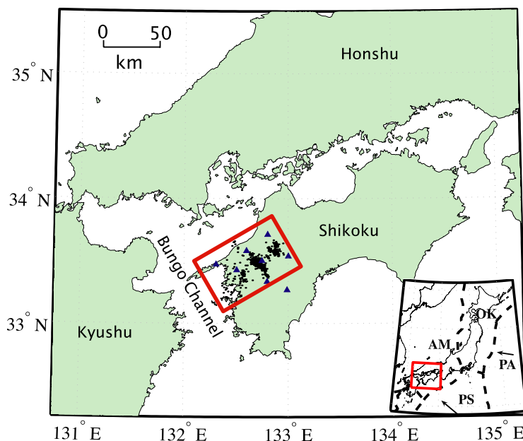
Figure 1. Tectonic setting and location of study area. Red box in main figure shows location of study area and denotes the region shown in Figures 3–16, parts a and b. Black dots indicate LFE template events. Blue triangles show the locations of the eight Hi-net stations used in this study. Inset shows the regional tectonics with the red box indicating the region shown in the main figure. Dashed lines indicate approximate plate boundaries. PA, Pacific plate; PS, Philippine Sea plate; AM, Amur plate; OK, Okhotsk plate.
